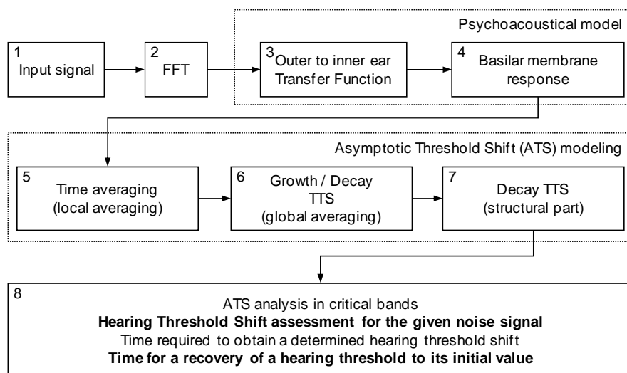
Fig. 2. Block diagram of a psychophysiological noise dosimeter.
